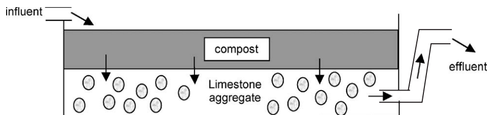
Fig. 5. Schematic layout of a reducing and alkalinity producing system (RAPS), redrawn after Younger et al. (2003). Water flowing through the compost layer is stripped of dissolved oxygen, while both this layer and the underlying limestone add alkalinity to the AMD.
