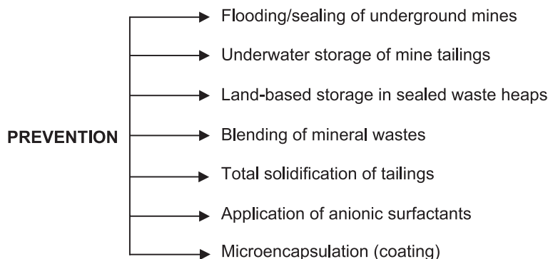
Fig. 1. Various approaches that have been evaluated to prevent or minimise the generation of mine drainage waters.
