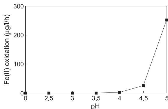
Fig. 4. Abiotic ferrous iron oxidation as a function of pH, calculated from Stumm and Morgan (1981) for an aqueous solution of 10 mM ferrous iron containing 8 mg O 2 /l.
