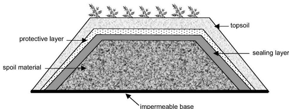
Fig. 2. Layout of a “dry cover” for minimising production of mine spoil effluents.
